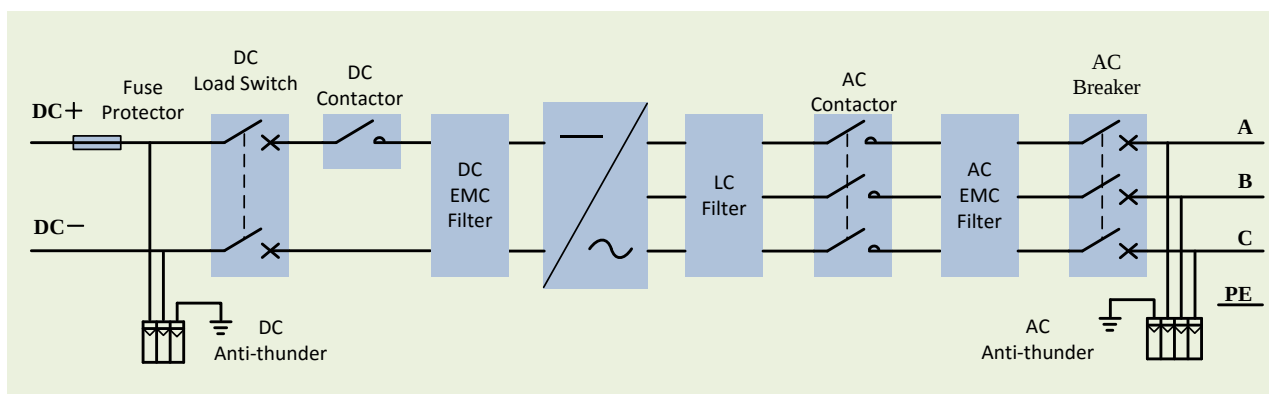
Figure 1: PCS Topology
