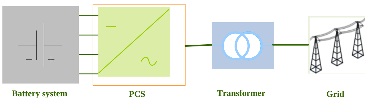
Figure 2: System Application
